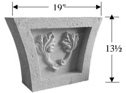
Projection=5" K#03
