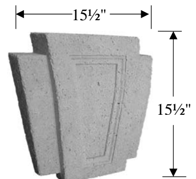
Projection=4 1/4" K#09
