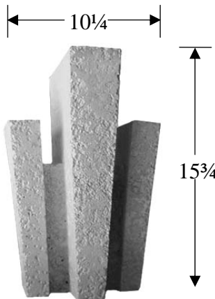
Projection=8 1/2" K#05
