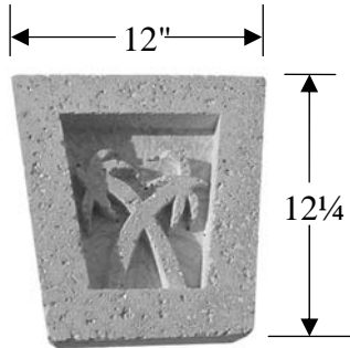
Projection=3 1/4" K#01
